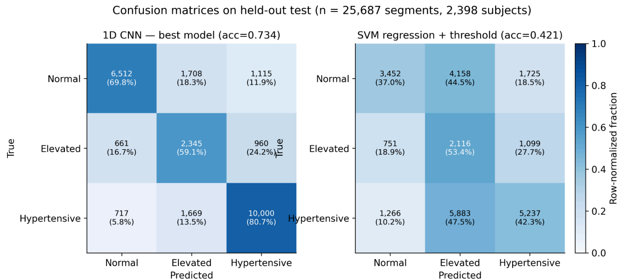
Figure 4. Row-normalized confusion matrices on the held-out test set for the best-performing 1D CNN and the support vector regression plus threshold baseline. The CNN shows strong diagonal performance with highest recall for hypertensive segments, whereas the regression-based baseline exhibits substantial confusion across classes, particularly misclassification of hypertensive cases as elevated.
