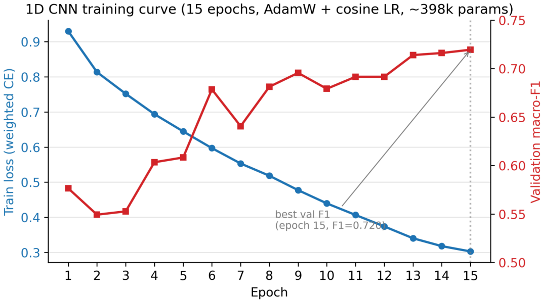
Figure 6: Training performance of the 1D CNN over 15 epochs.
