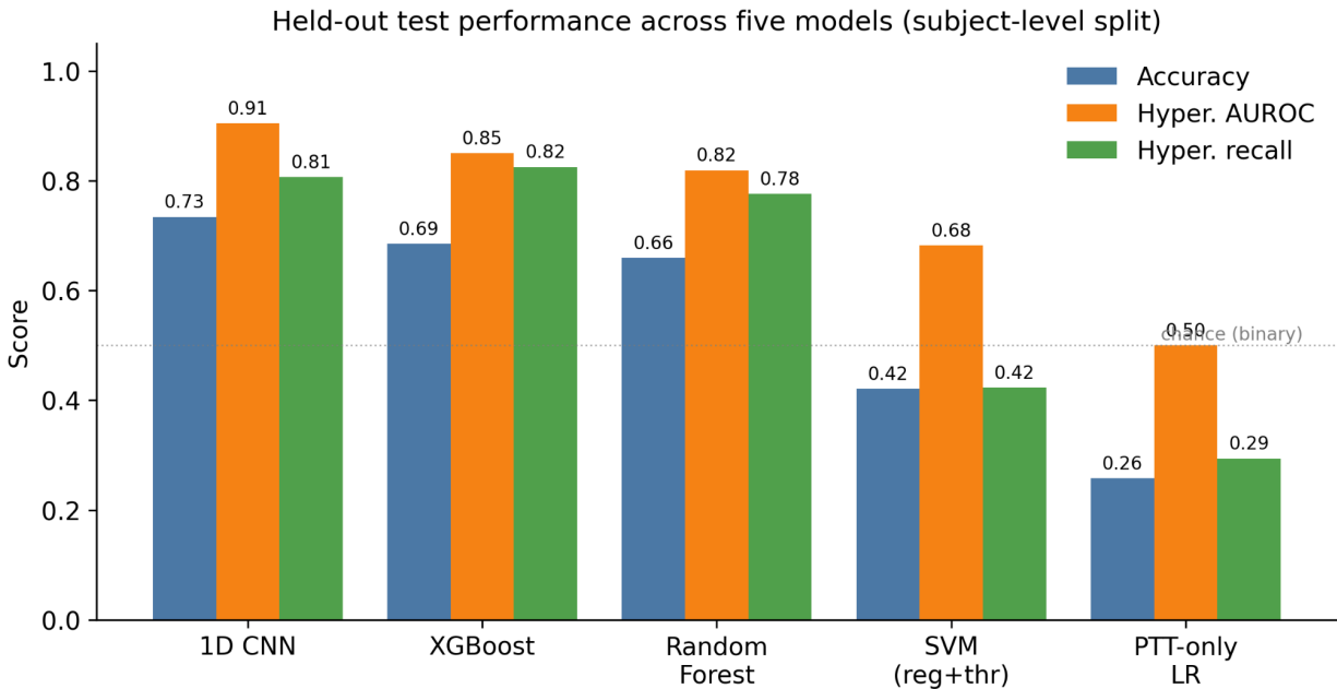
Figure 3. Held out test performance across five models. 1D-CNN achieved strongest overall performance, while XGBoost produced comparable results and highest hypertensive recall.
